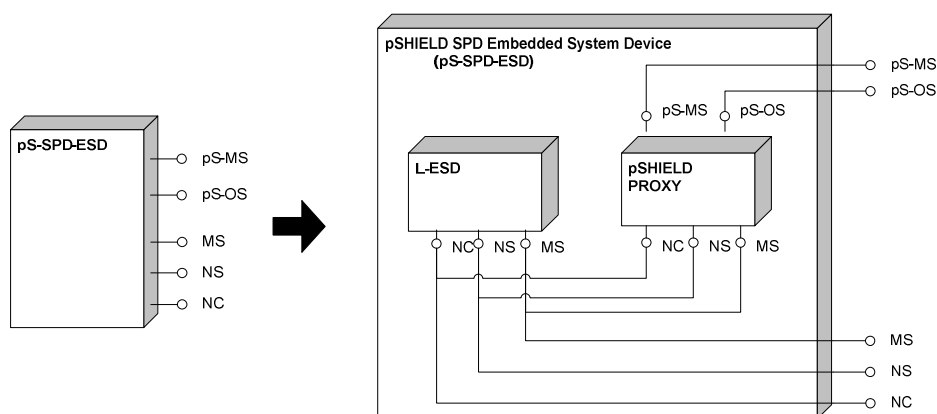
Figure 43 – pS-SPD-ESD architecture
