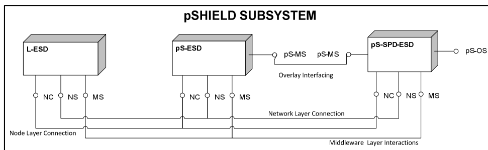
Figure 40 – pSHIELD Subsystem architecture decomposed into ESD components
