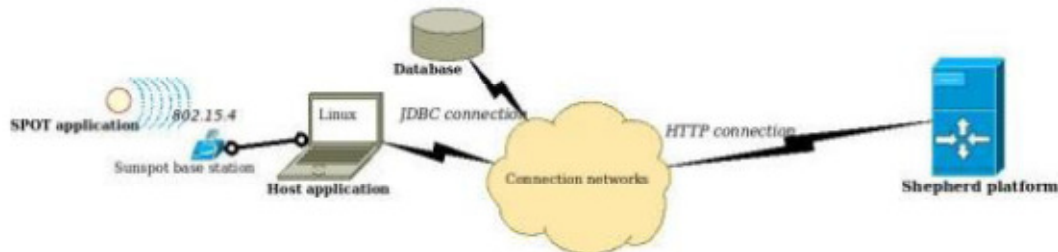
Figure 26 – Network of connected devices (M2M platform)
