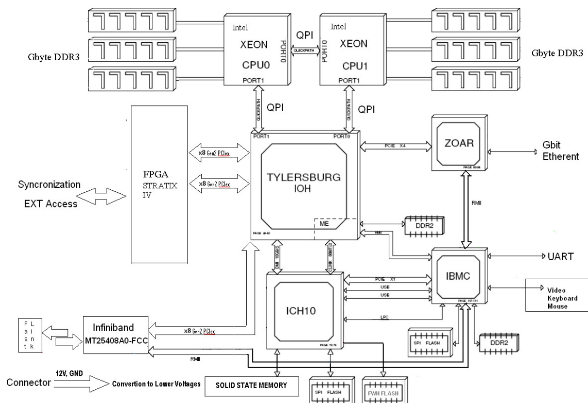
Figure 21 - Power Node architecture: high level description
