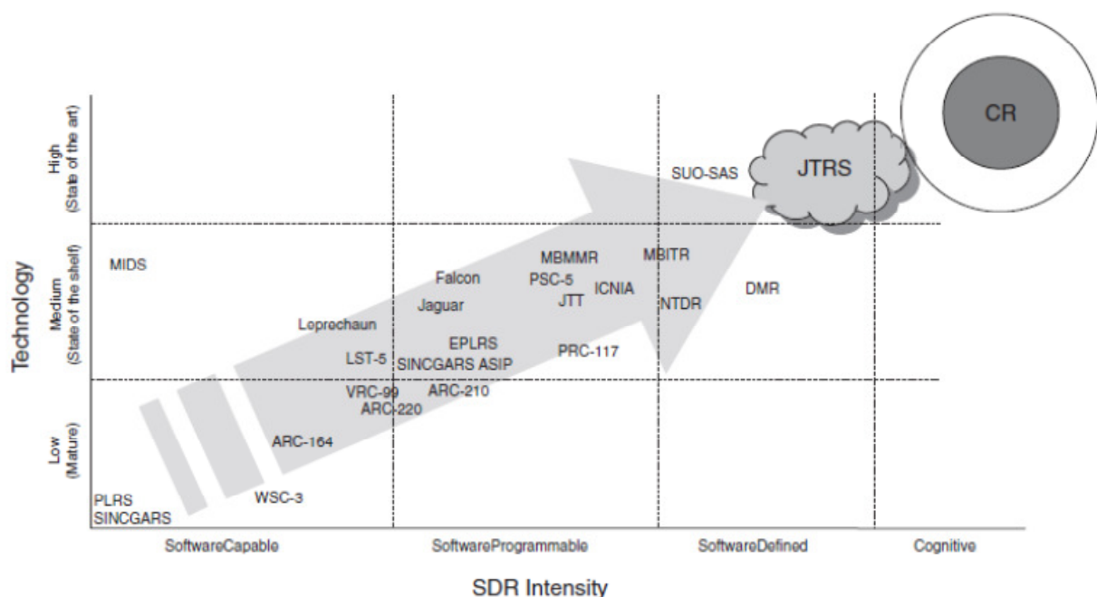
Figure 27 – SDR evolution
