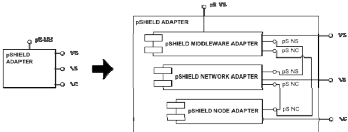
Figure 46 – pSHIELD Adapter component architecture
