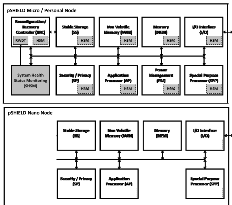
Figure 17 - Schematic view of SPD modules of a generic pSHIELD Nano, Micro and Personal Node
