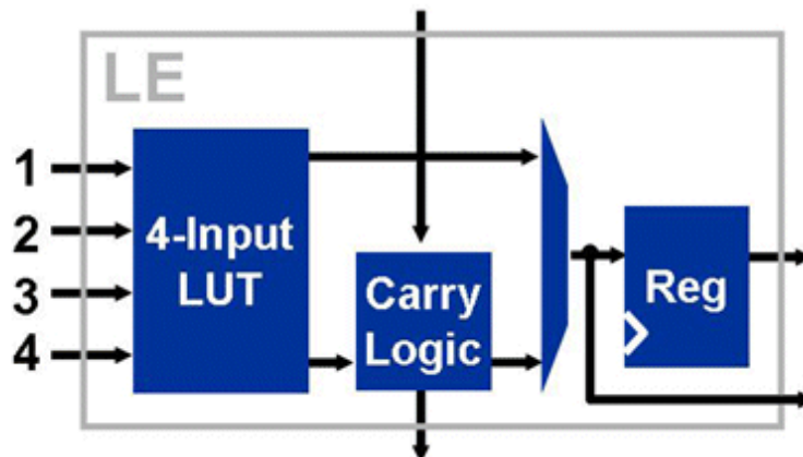
Figure 22 – Internal structure of an FPGA logic element
