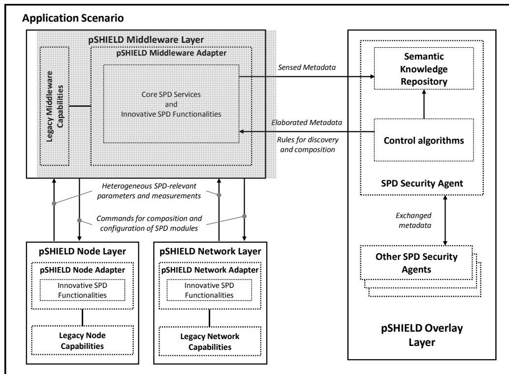
Figure 11 – pSHIELD Middleware layer
