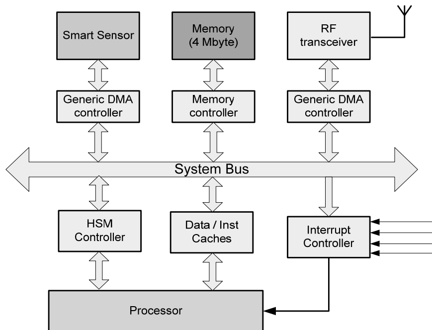
Figure 18 - Hardware architecture and nano node chip partitioning
