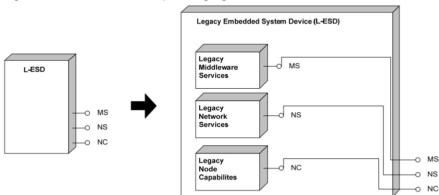
Figure 49 – L-ESD component architecture
