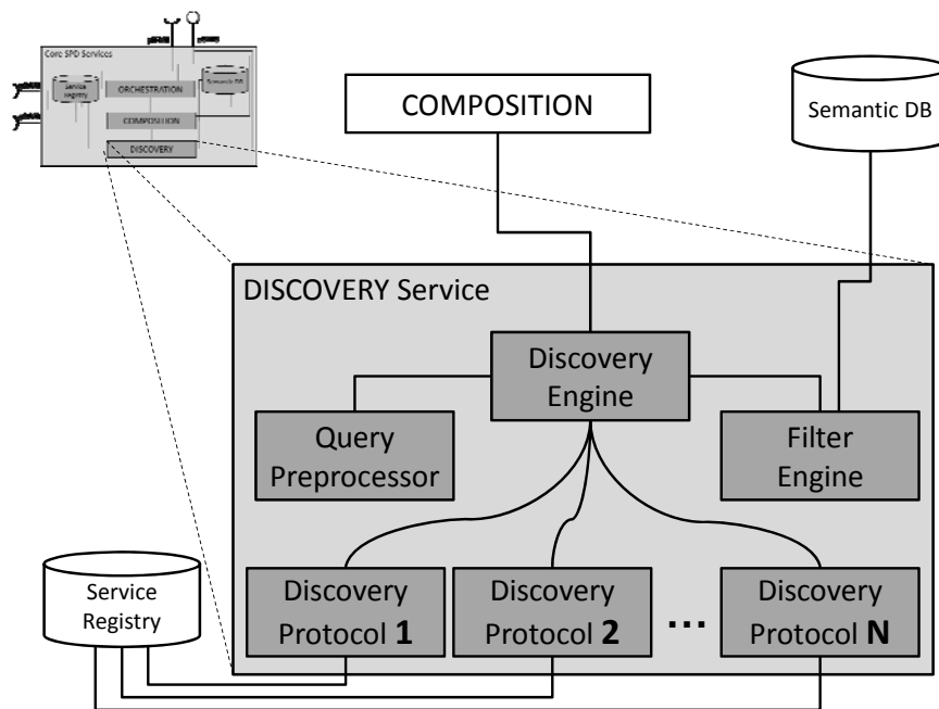
Figure 32 – Details of the Discovery core SPD service
