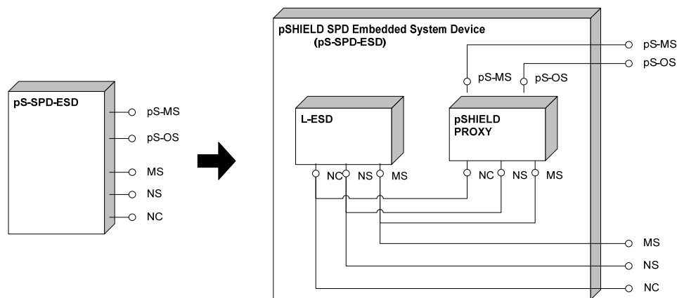
Figure 43 – pS-SPD-ESD architecture
