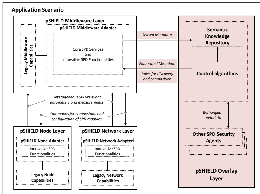
Figure 33 – pSHIELD overlay: a functional view
