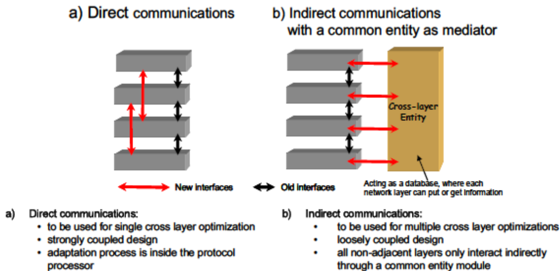
Figure 7 - Cross-layer architectures for indirect and direct communications
