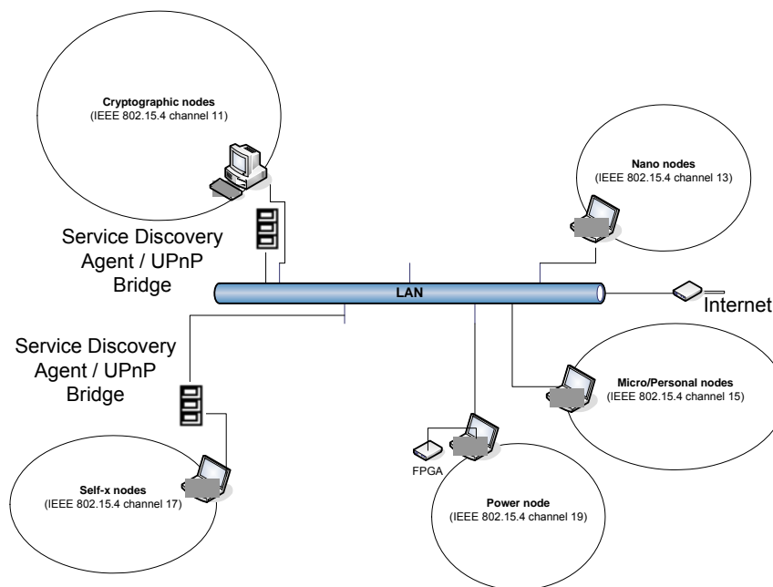
Figure 10 - Network Layer: paradigm architecture
