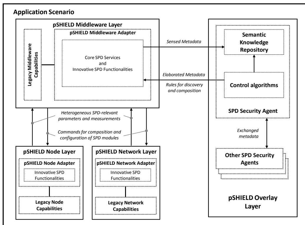
Figure 50 – pSHIELD functional component architecture
