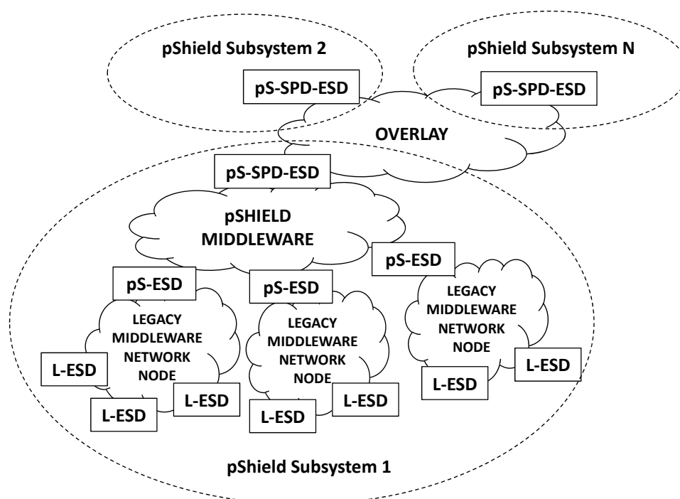
Figure 42 – pSHIELD System Architecture highlighting the ESD types
