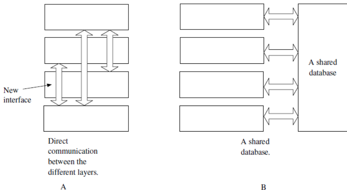
Figure 4 - Proposals for architectural blueprints for wireless communications
