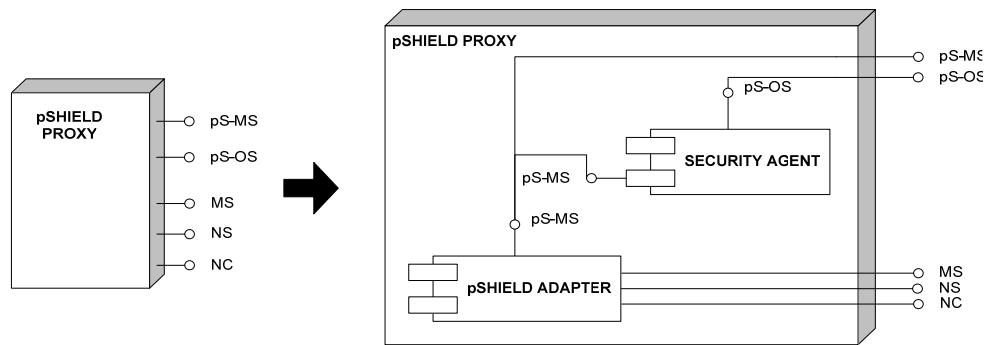
Figure 44 – pSHIELD Proxy component architecture
