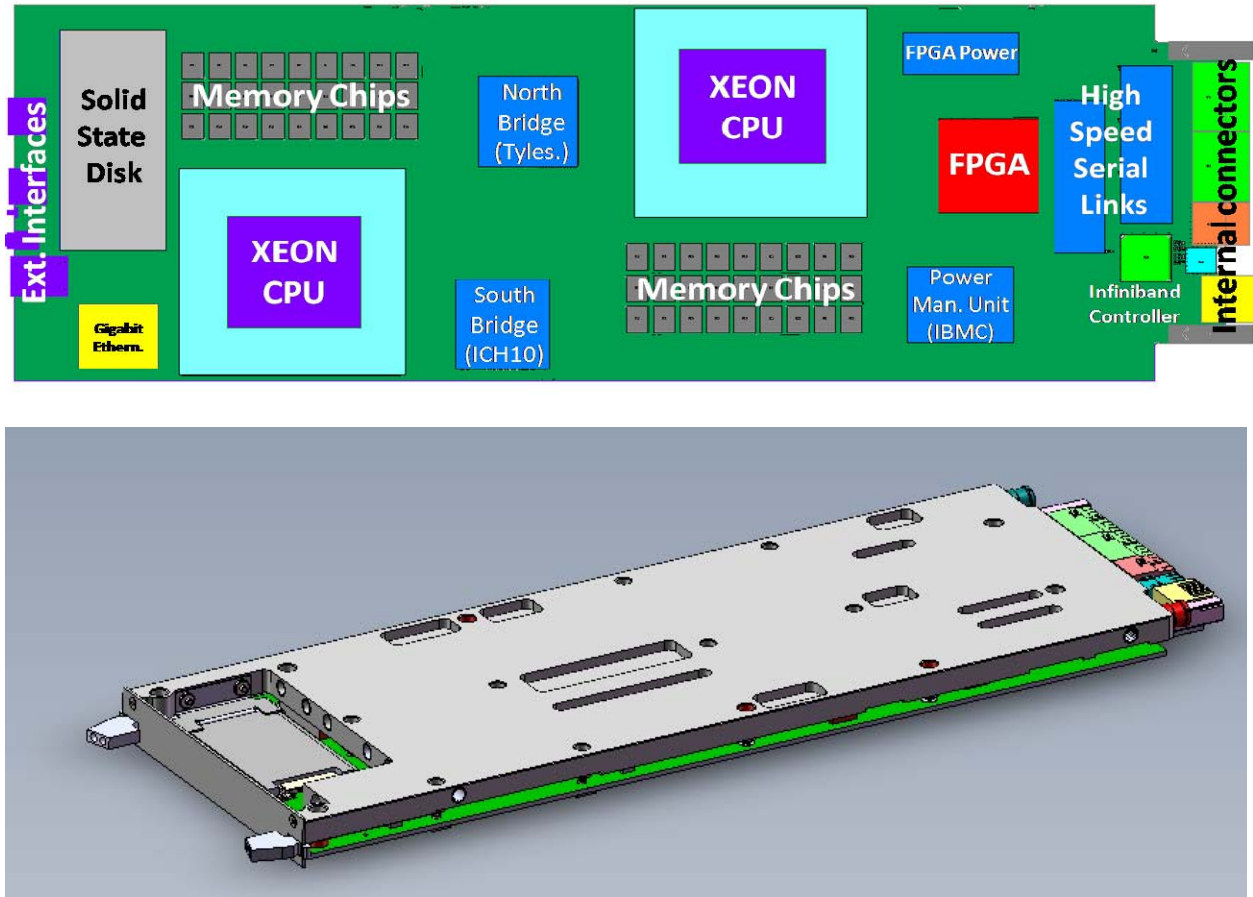
Figure 20 - Power Node board concept, with and without cooling heat sinks
