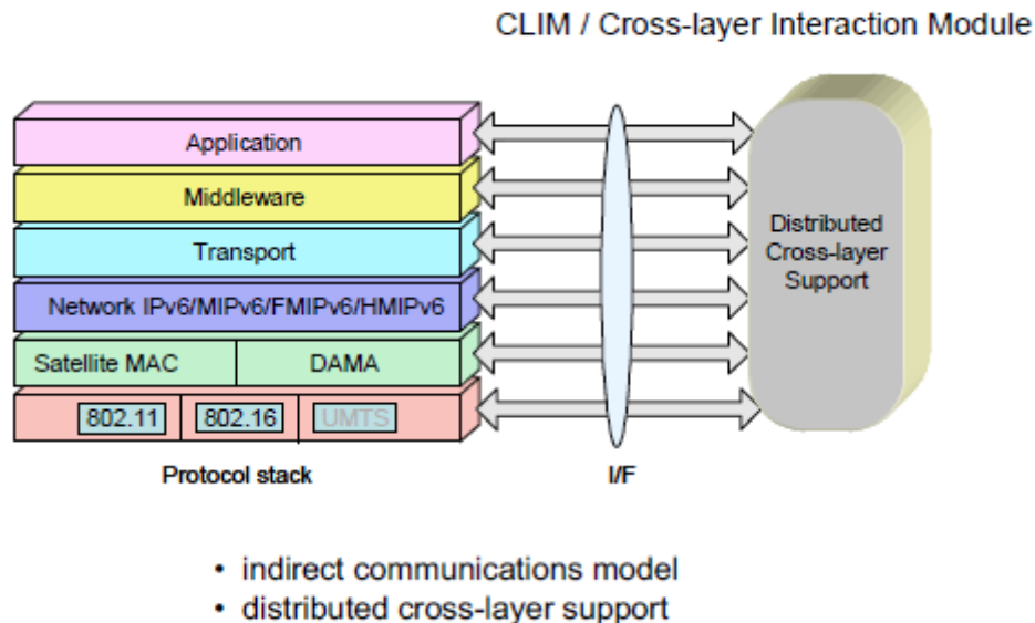
Figure 5 - Proposed Cross-Layer Interaction Model
