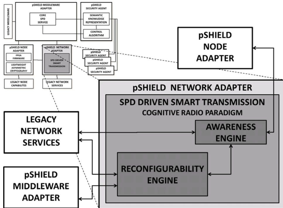
Figure 28 – pSHIELD NETWORK ADAPTER conceptual model
