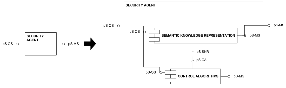
Figure 45 – pSHIELD Security Agent component architecture
