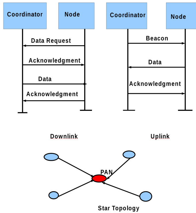
Figure 6.1: Beacon transmission in Star topology, is updated from [30]
