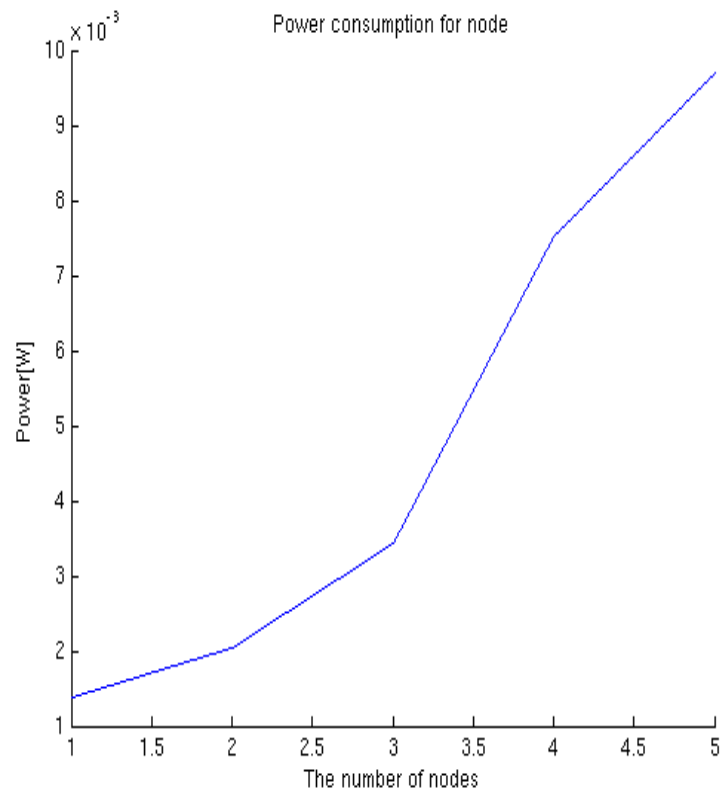
Figure 7.6: Power consumption for each node in Mesh topology .
