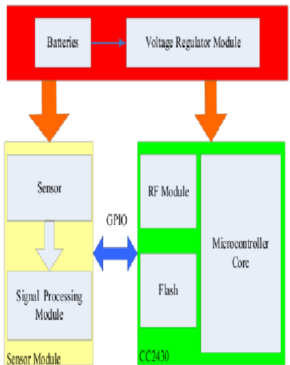
Figure 5.6: The basic units of a sensor node [24]
