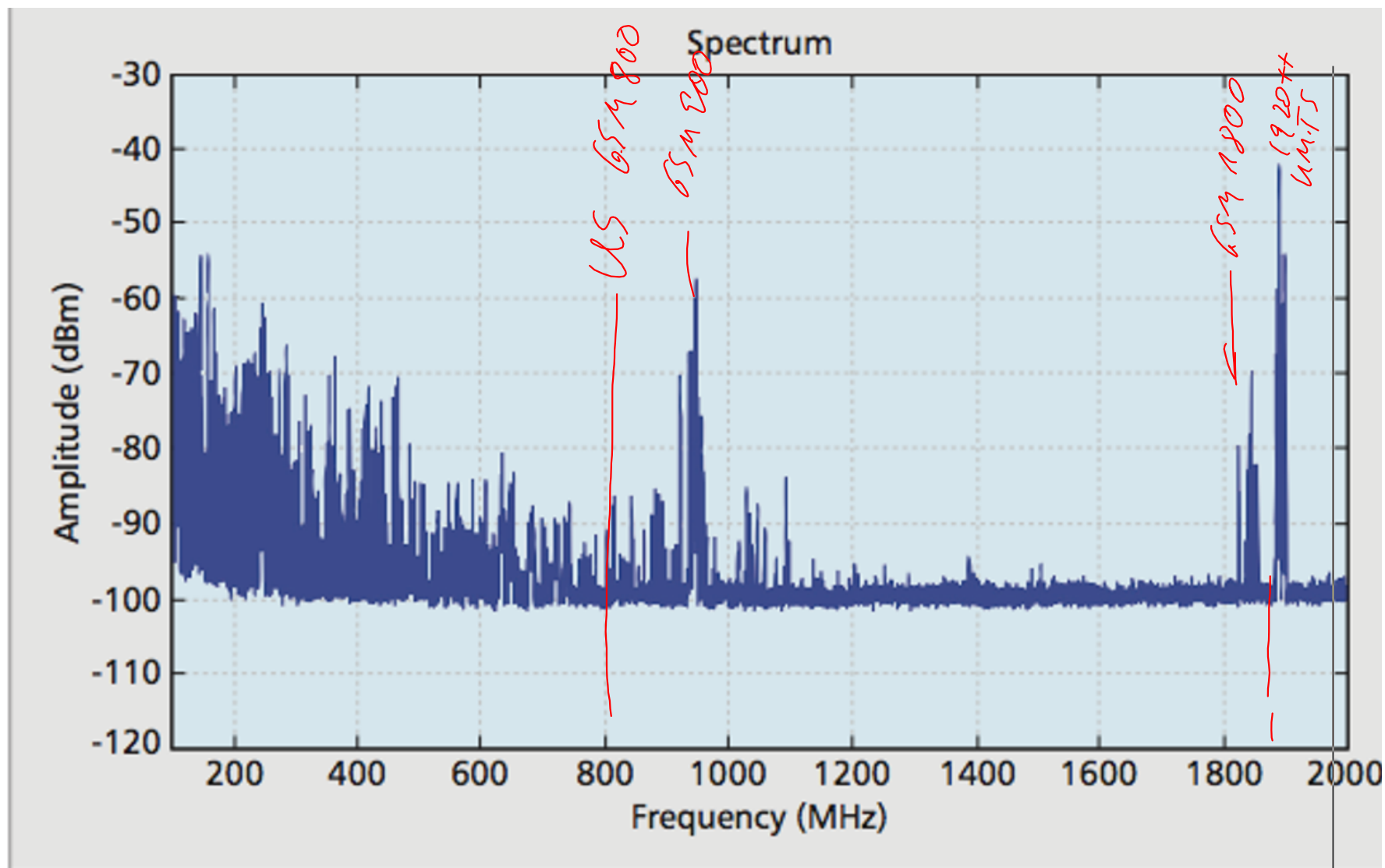
Figure 1. Electromagnetic interference measured in a boiler house.
