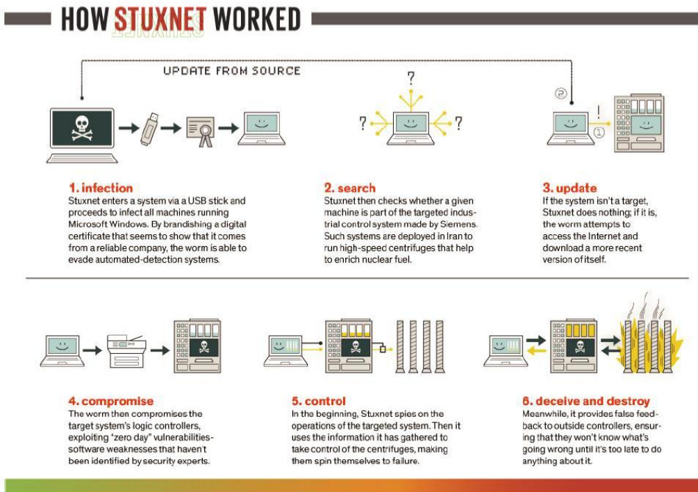
Figure 2: How Stuxnet worked [10].
