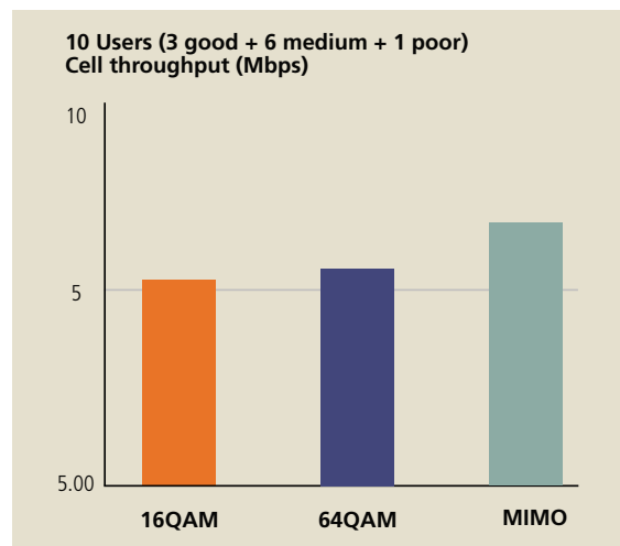
Figure 4.1: Field Test, Relative Average Cell Gain of MIMO Compared to 16 QAM and to 64 QAM
