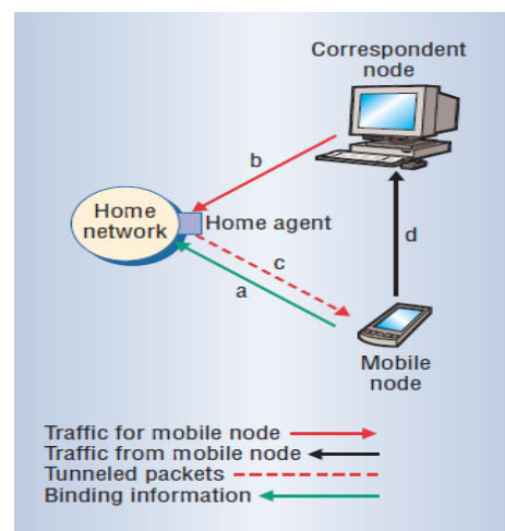
Figure1. The operation of MIPv4
